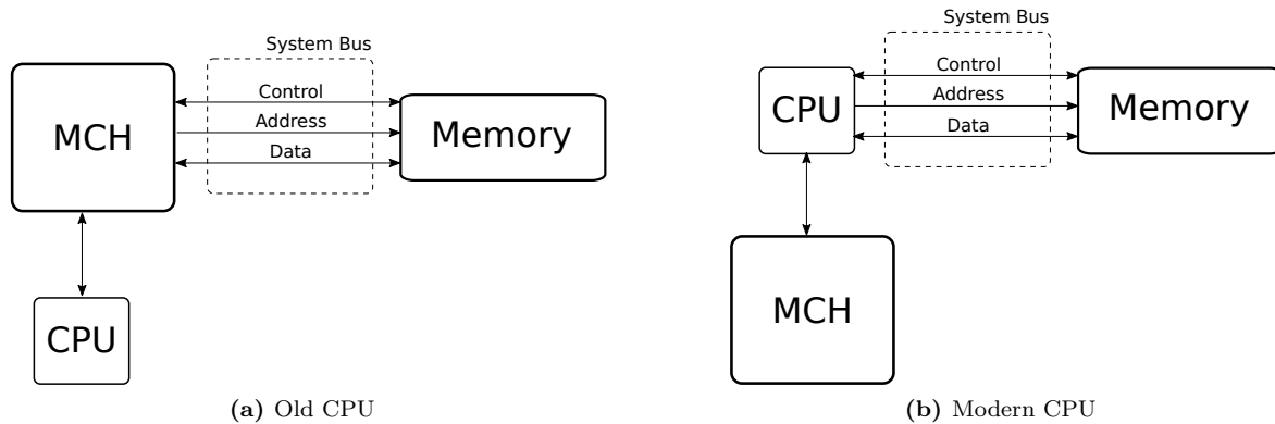
Figure 3.2.2: CPU - Memory Communication
