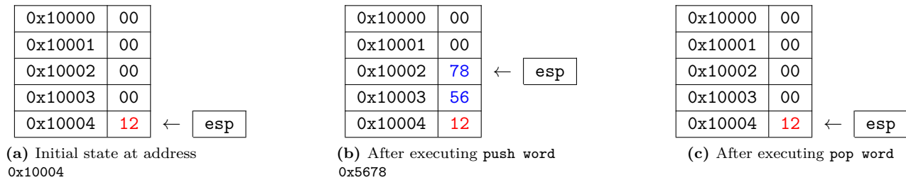
Figure 4.9.4: Stack operations
