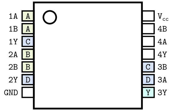
(b) Pin layout; pin 3A and 3B take the values from 1Y and 2Y.
